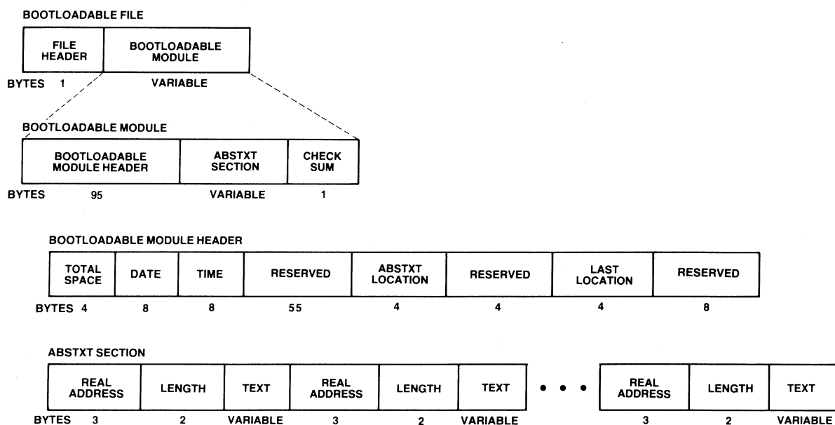
Figure B-1 286 Absolute Bootloadable File Format
